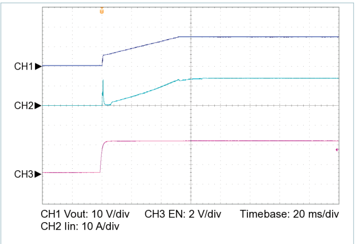
Figure 17 — Startup from EN, V_{IN} = 24\text{ V} , C_{OUT\_EXT} = 6800\text{ }\mu\text{F} , R_{LOAD} = 0.701\text{ }\Omega
