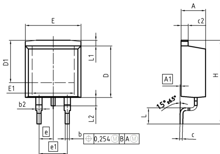
PG-TO263-3
