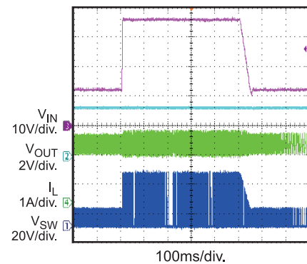
Load Dump
