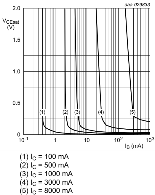
Fig. 9. Collector-emitter saturation region as a function of base current; typical values
