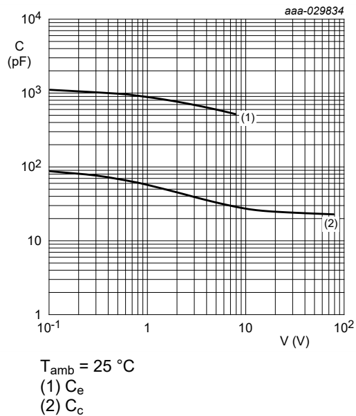
Fig. 10. Input/output capacitance as a function of input/output voltage
