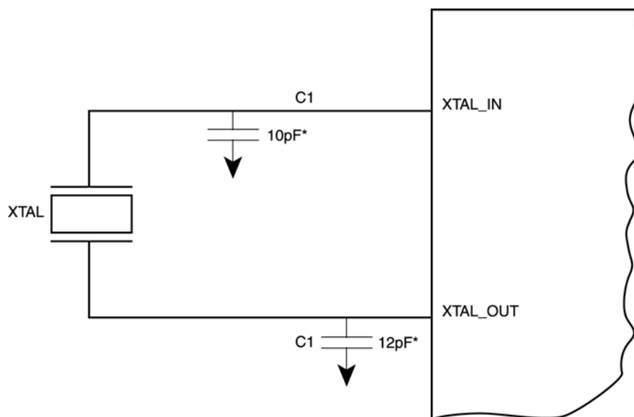
Figure 3 Crystal with Trim Caps
