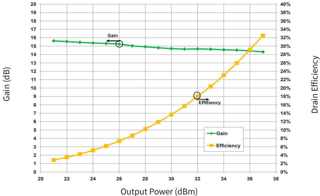
Typical Gain and Efficiency versus Output Power measured in CGH27030F-AMP V_{DD} = 28\text{ V} , I_{DQ} = 150\text{ mA} , 802.16-2004 OFDM, PAR=9.8 dB
