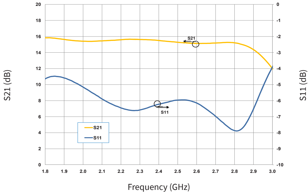
Small Signal S-Parameters vs Frequency measured in CGH27030F-AMP V_{DD} = 28\text{ V}, I_{DQ} = 150\text{ mA}
