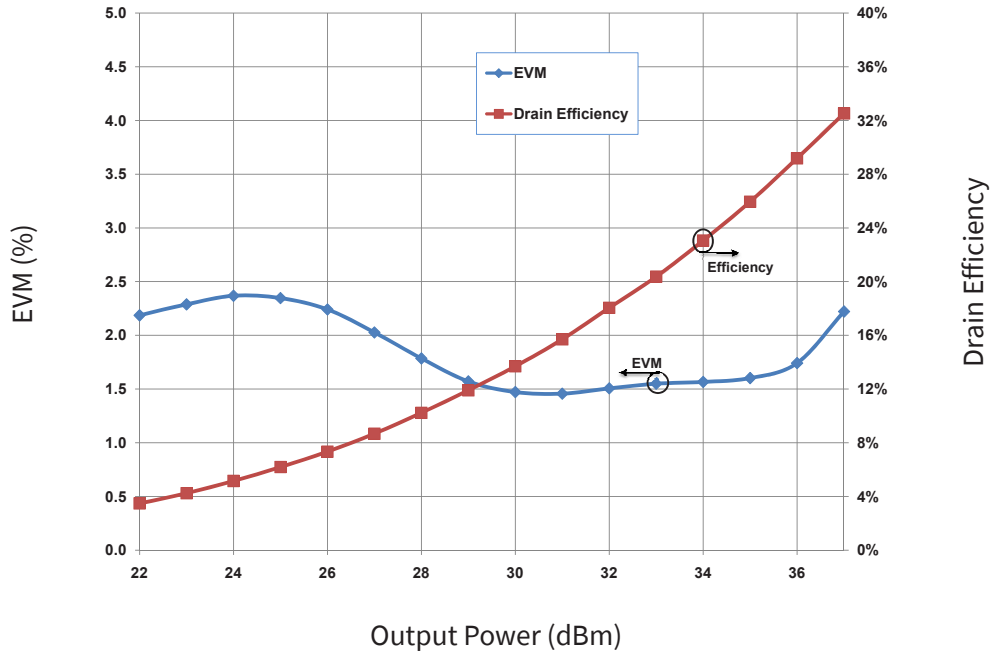
Drain Efficiency and EVM vs Output Power measured in CGH27030F-AMP V_{DD} = 28\text{ V} , I_{DQ} = 150\text{ mA} , 802.16-2004 OFDM, PAR = 9.8 dB
