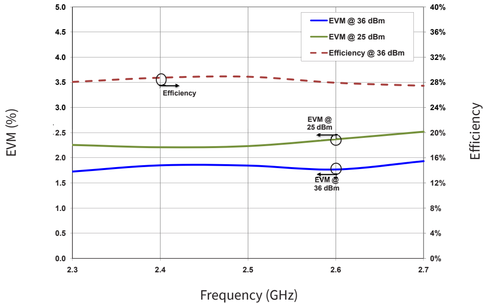
Typical EVM and Efficiency versus Frequency measured in CGH27030F-AMP V_{DD} = 28\text{ V}, I_{DQ} = 150\text{ mA}, 802.16\text{-}2004\text{ OFDM}, \text{PAR} = 9.8\text{ dB}, P_{AVE} = 5\text{ W}
