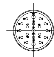
19-Pole (16+3)
