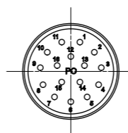
16-Pole
