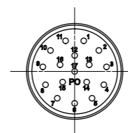
17-Pole (16+1)
