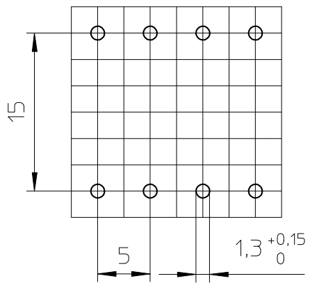
Hole pattern:
