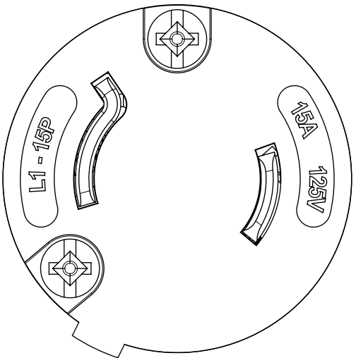
FACE VIEW
