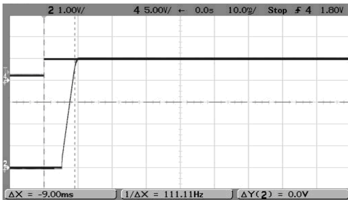
On/Off Enable Delay (Vin=13.8V, Vout=5V, Iout=6.1A, Load=0) Trace 4=Enable, Trace 2=Vout
