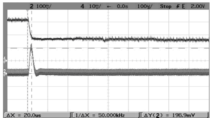
Step Load Transient Response (Vin=12V, Vout=5V, Load=0, Iout=6A to 3A) Trace 2=Vout, 100 mV/div. Trace 4=Iout, 2A/div.
