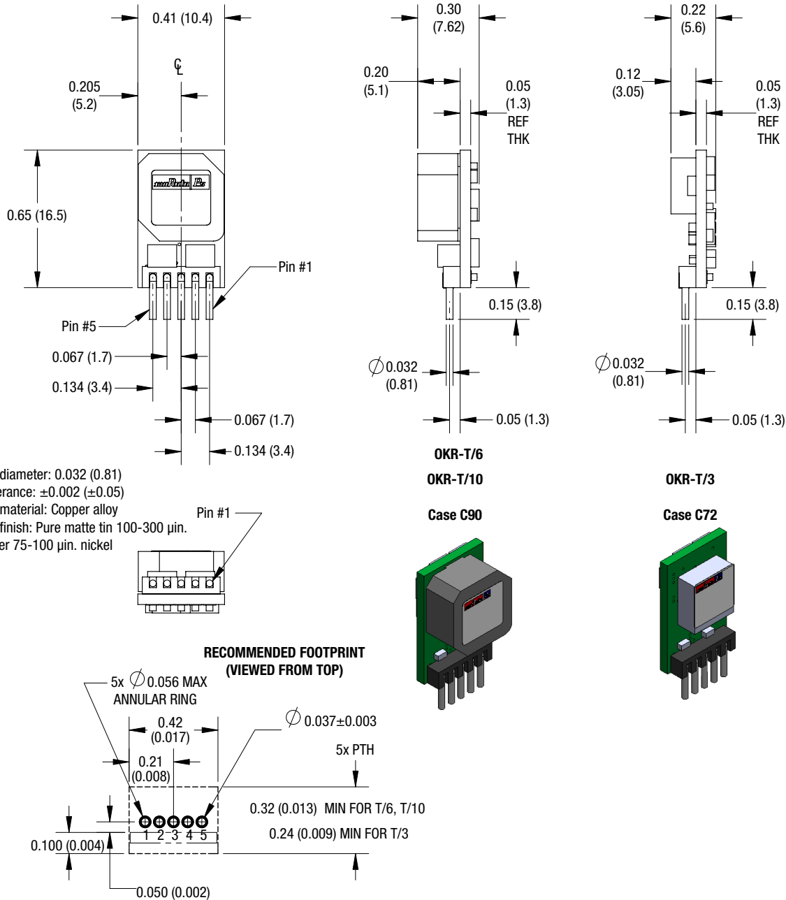
Figure 2. OKR Series Component locations are typical.
