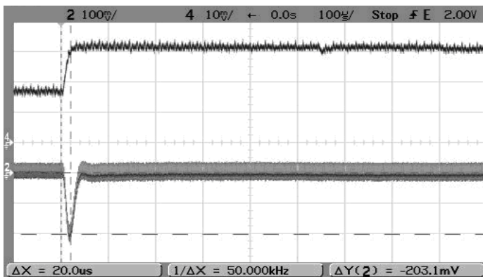
Step Load Transient Response (Vin=12V, Vout=5V, Load=0, Iout=3A to 6A) Trace 2=Vout, 100 mV/div. Trace 4=Iout, 2A/div.
