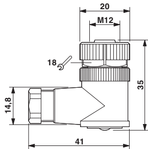
Dimensional drawing
