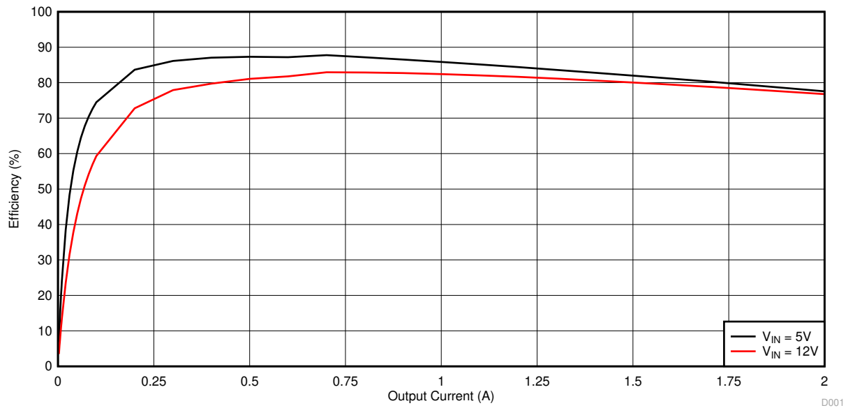
Figure 4-1. TPS562219AEVM-663 Efficiency
