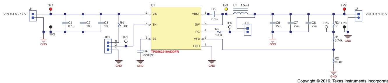
Figure 6-1. TPS562219AEVM-663 Schematic Diagram
