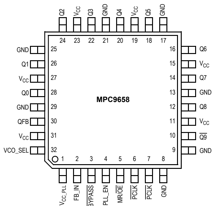
Figure 2. MPC9658 32-Lead Pinout (Top View)
