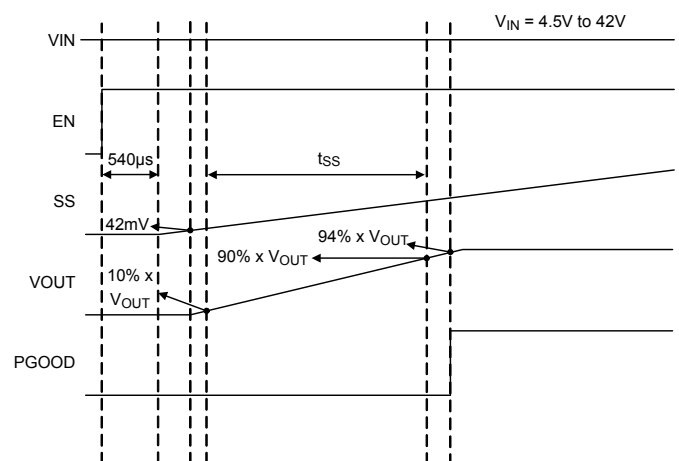
Figure 1 Start-Up Sequence for RT6345GQW
