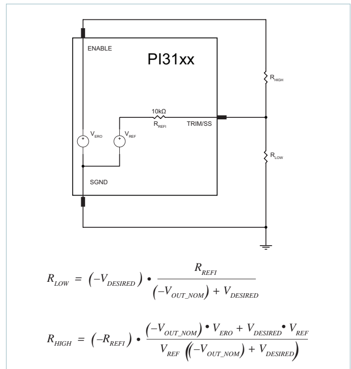
Figure 42 — Trim equations and equivalent circuit
