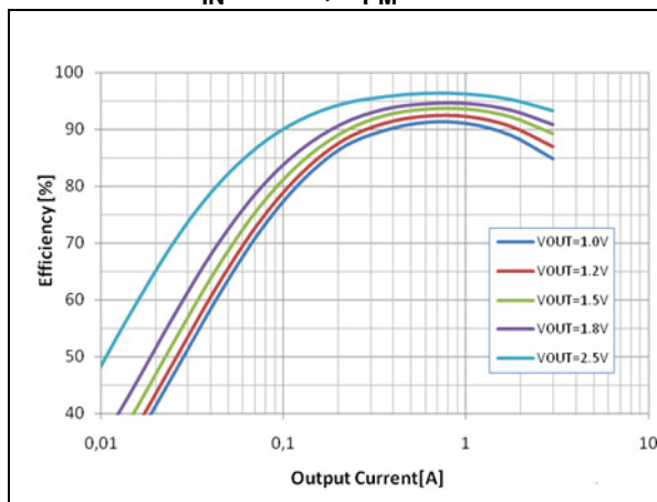
Figure 4. Efficiency vs. output current - V_{IN} = 3.3\ V , R_{PM} = 240\ k\Omega
