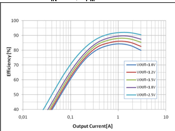
Figure 5. Efficiency vs. output current - V_{IN} = 5\ V , R_{PM} = 240\ k\Omega
