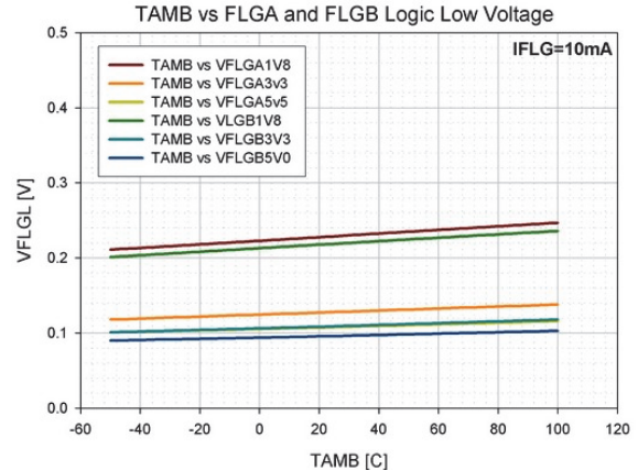
Fig. 9: FLG Logic Low Voltage vs. Temperature
