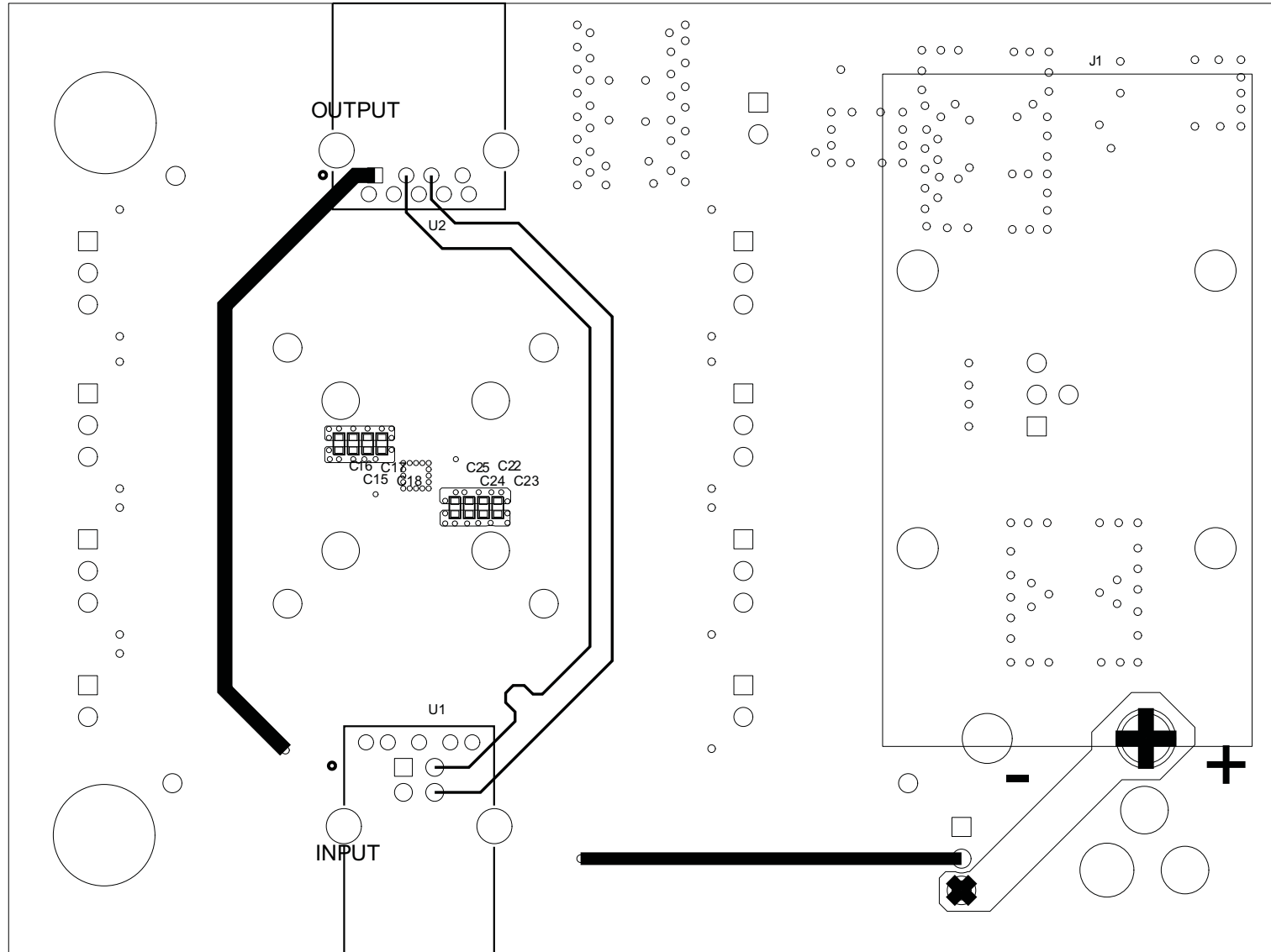
Figure 14. SN65LVPE502CP EVM Layout Layer 6 (Bottom)
