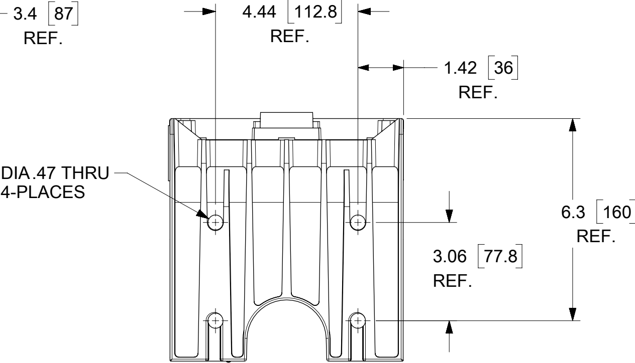
BOTTOM VIEW
