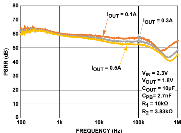
FIGURE 2. PSRR
