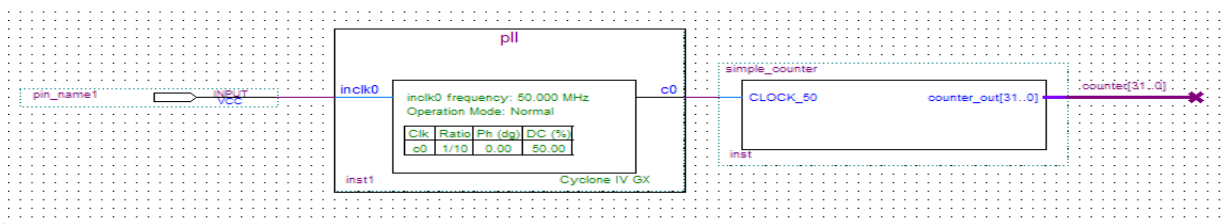
Figure 3-18 Connecting the PLL symbol and Input port
