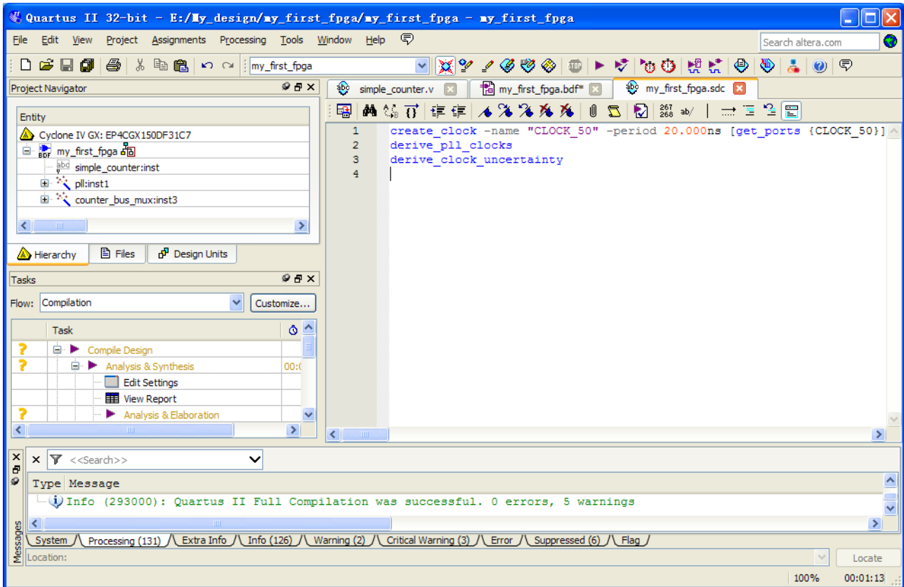
Figure 3-32 Default SDC
