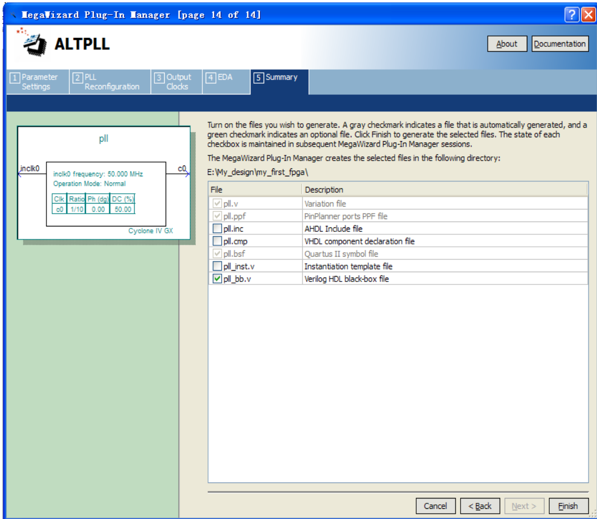
Figure 3-13 Wizard-Created Files
