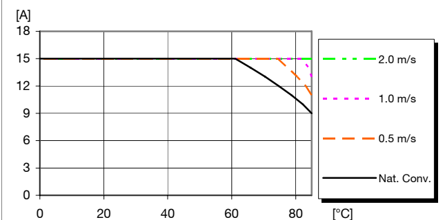
Available load current vs. ambient air temperature and airflow at V_I = 3.3\text{ V} , V_{OUT} = 2.5\text{ V} . See Thermal Consideration section.
