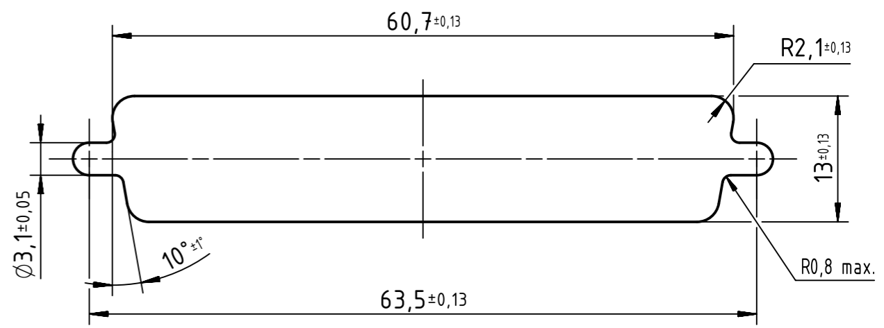
Front mounting panel cut out
