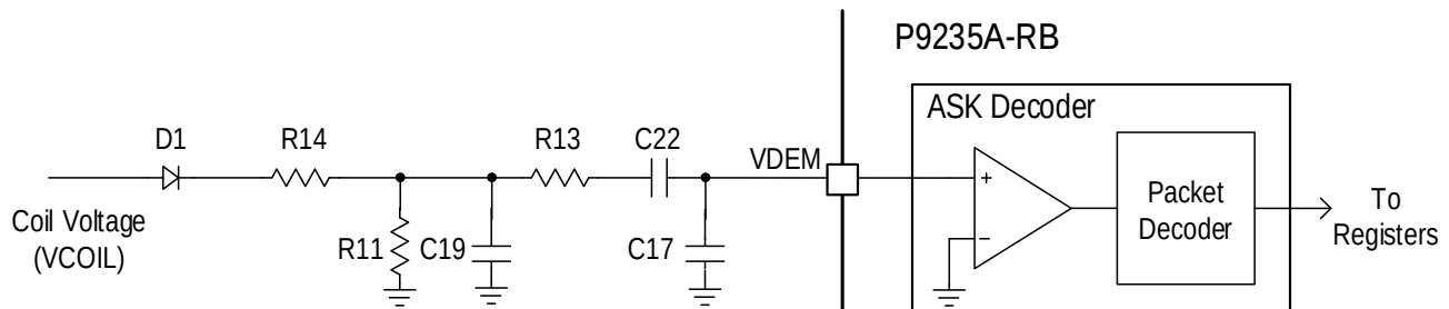
Figure 4. Voltage Mode Envelope Detector
