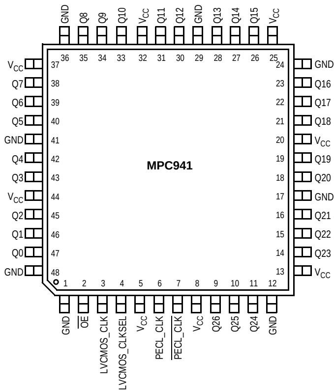
Pinout: 48-Lead TQFP (Top View)
