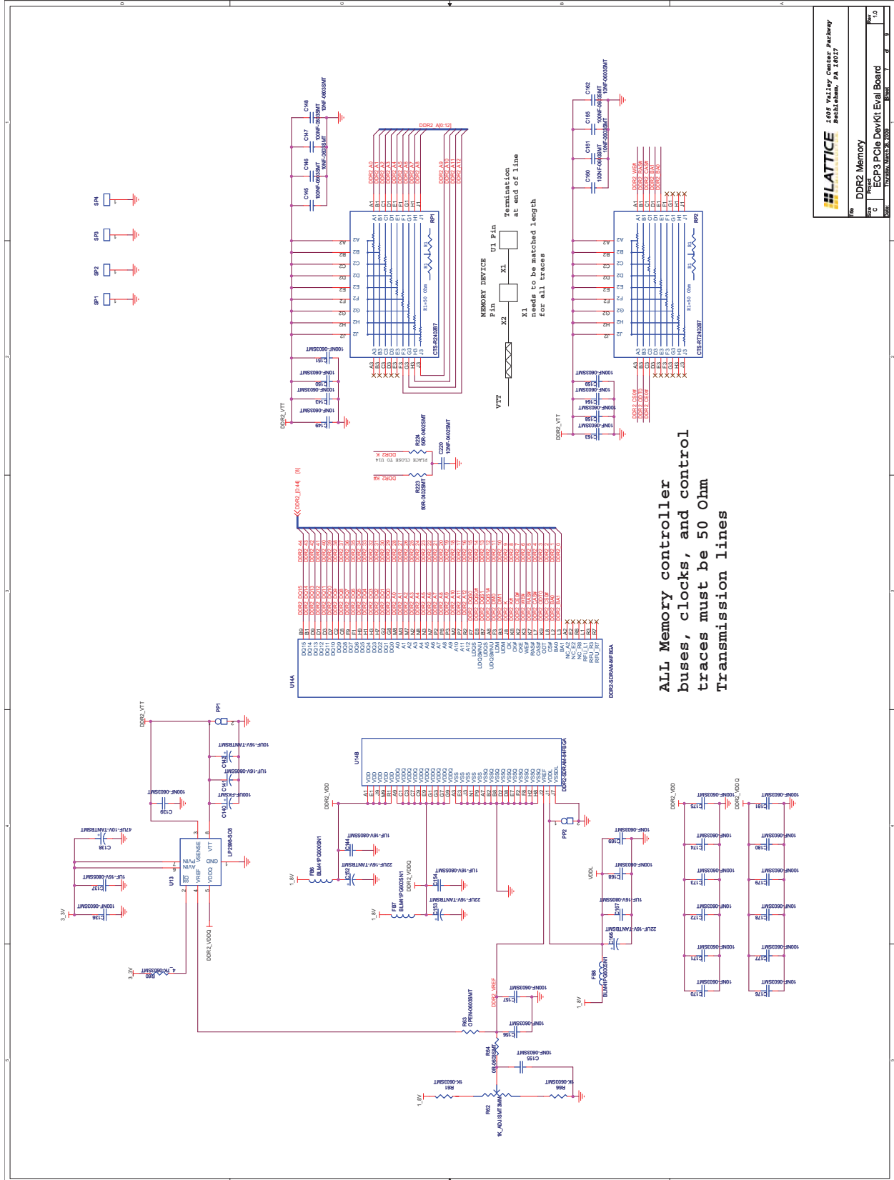
Figure 26. DDR2 Memory
