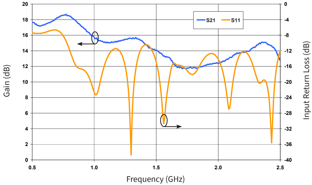
Gain and Input Return Loss vs Frequency from 0.5 GHz to 2.5 GHz in Broadband Amplifier Circuit CGH40090PP-AMP V_{DD} = 28\text{ V}, I_{DQ} = 1.0\text{ A}
