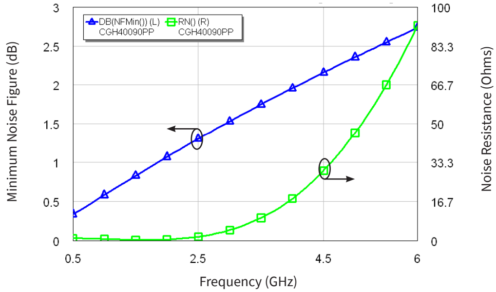
Simulated Minimum Noise Figure and Noise Resistance vs Frequency of the CGH40090PP V_{DD} = 28\text{ V}, I_{DQ} = 500\text{ mA (per side)}
