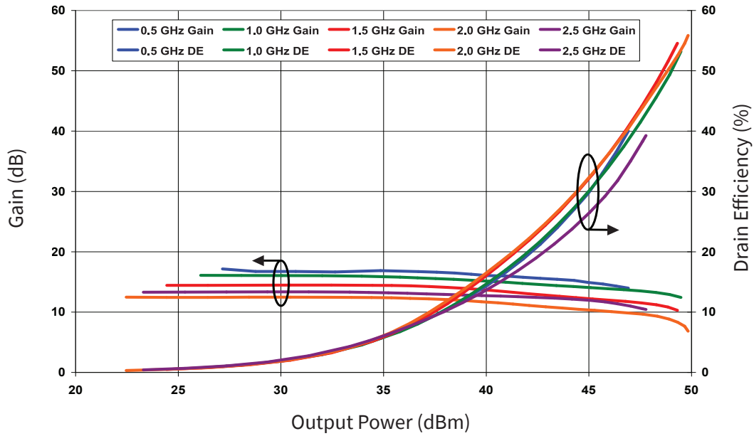
Gain and Efficiency vs Output Power measured in Broadband Amplifier Circuit CGH40090PP-AMP V_{DD} = 28\text{ V}, I_{DQ} = 1.0\text{ A}, \text{Freq} = 0.5 - 2.5\text{ GHz}
