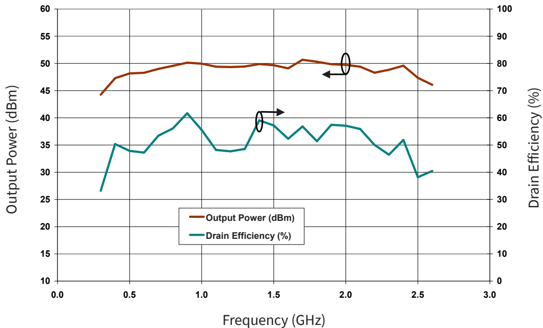
Output Power and Drain Efficiency vs Frequency measured in Broadband Amplifier Circuit CGH40090PP-AMP V_{DD} = 28\text{ V}, I_{DQ} = 1.0\text{ A}
