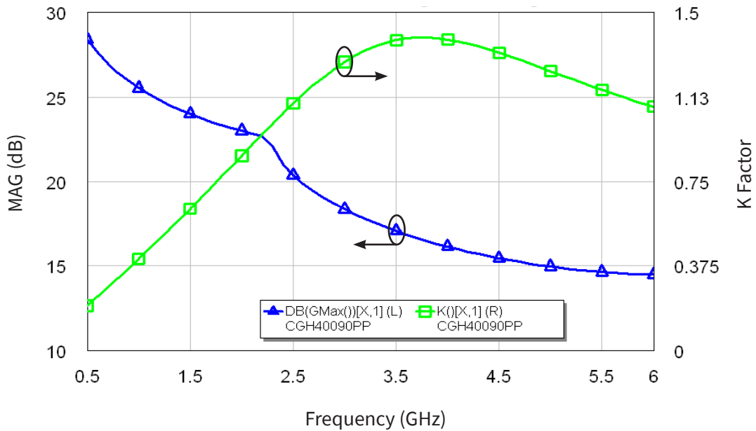
Maximum Available Gain and K Factor of the CGH40090PP V_{DD} = 28\text{ V}, I_{DQ} = 1.0\text{ A}
