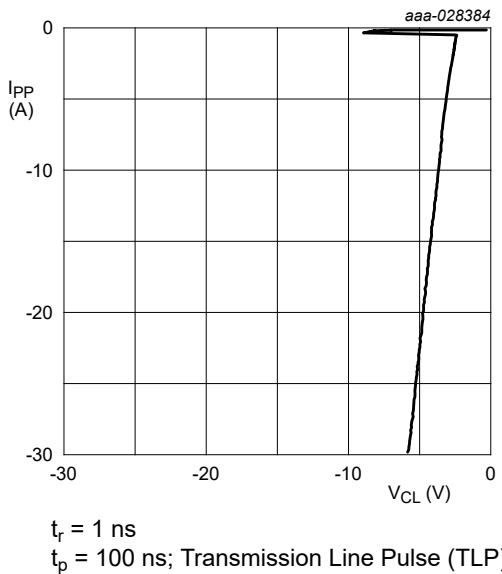
Fig. 4. Dynamic resistance with negative clamping; typical values
