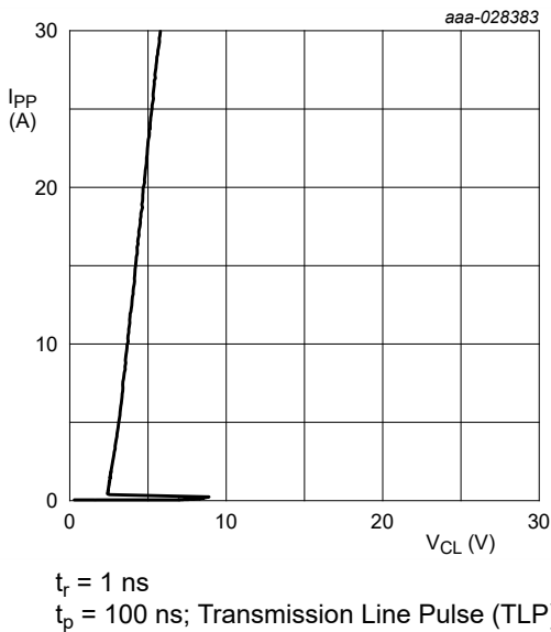
Fig. 3. Dynamic resistance with positive clamping; typical values
