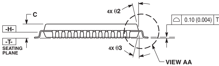
VIEW AA
