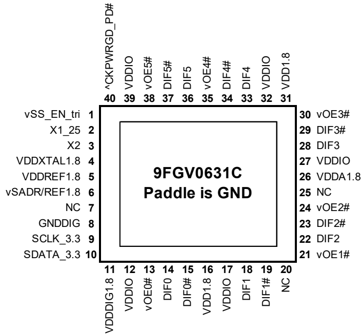
40-VFQFPN, 5 x 5 mm, 0.4mm pitch
