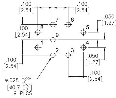
9 PIN
