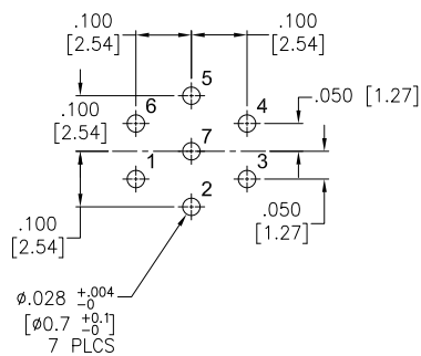
7 PIN
