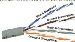
Straight-Through Cable Pin Out for T568B
