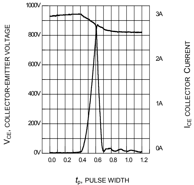
Figure 20. Typical turn off behavior, hard switching ( V_{GE} = 15/0V, R_G = 82\Omega, T_j = 150^\circ C , Dynamic test circuit in Figure E)
