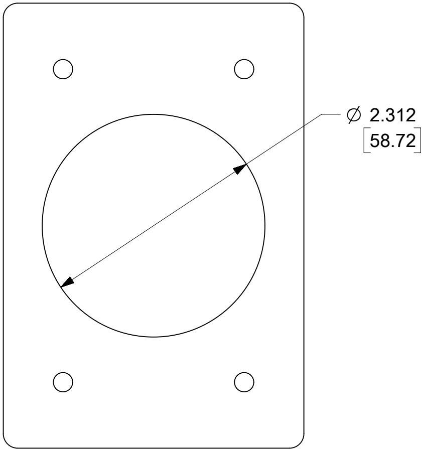
CLEARANCE HOLE (FOR PANEL MOUNT)
