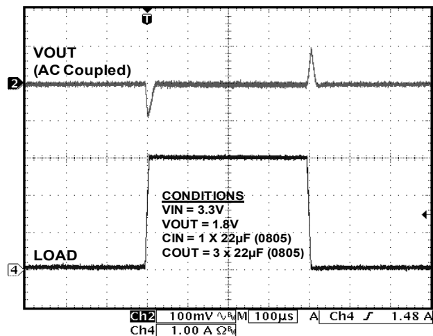
Load Transient from 0 to 3A
