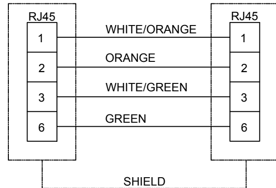
WIRING DIAGRAM
