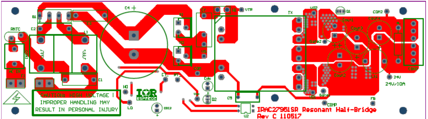
Figure 5 - Board Top Layer Copper
