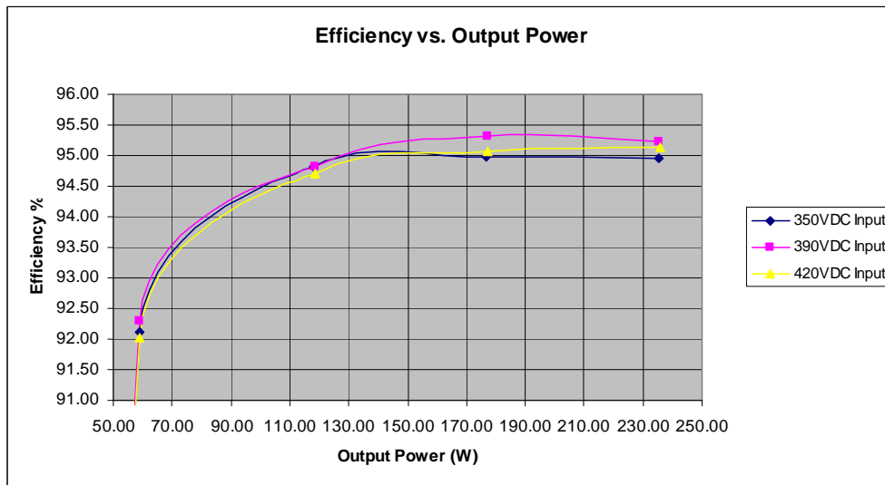
Figure 9 - Efficiency plot
