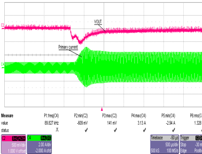
No Load to Full Load Step at 390Vdc
