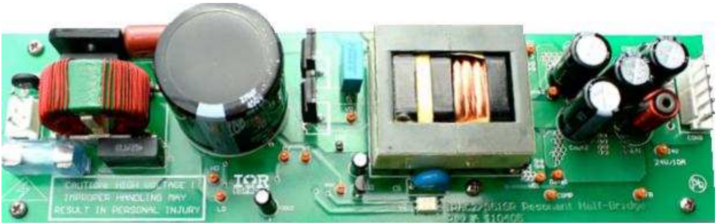
Figure 2 – Evaluation Board Photo
