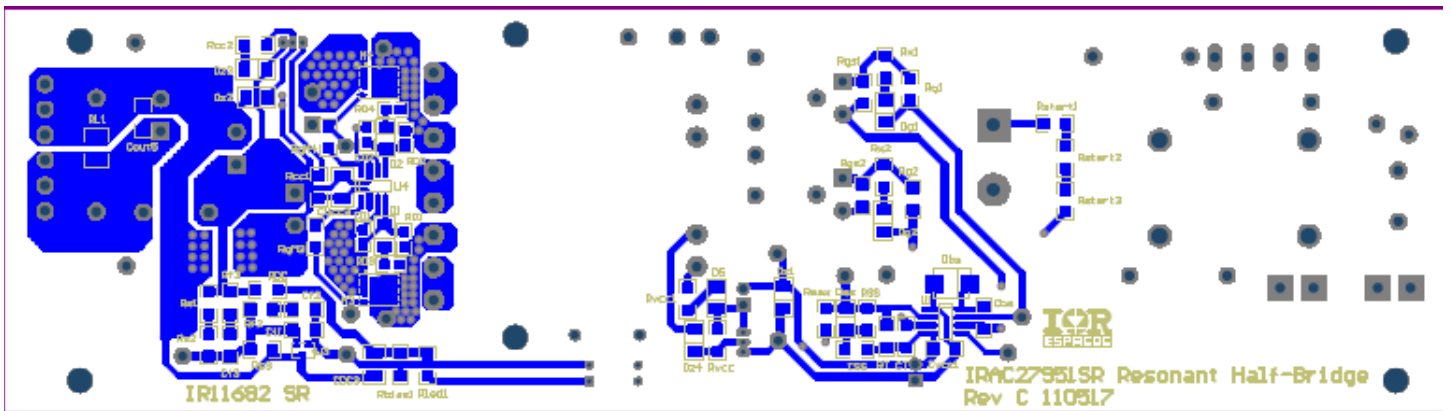
Figure 6 - Board Bottom Layer Copper
