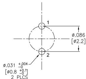
2 PIN
