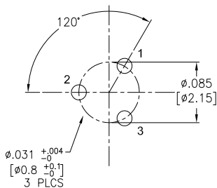
3 PIN
