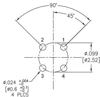
4 PIN
