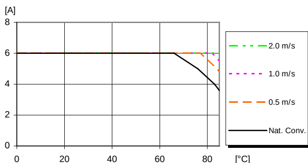
Available load current vs. ambient air temperature and airflow at V_I = 12.0 V , V_{OUT} = 3.3 V . See Thermal Consideration section.
