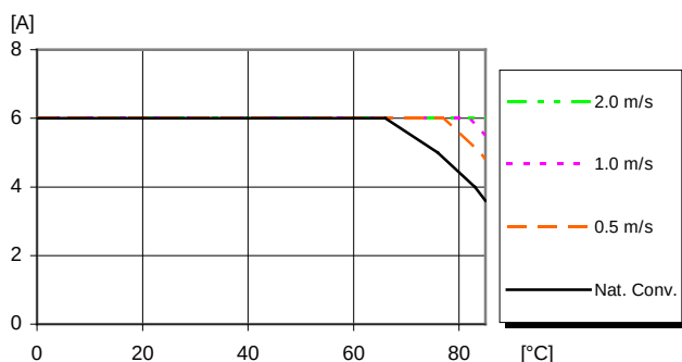
Available load current vs. ambient air temperature and airflow at V_I = 12.0\text{ V} , V_{OUT} = 3.3\text{ V} . See Thermal Consideration section.
