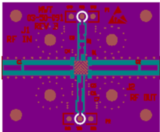
Figure 1 Evaluation Board
