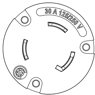
FACE VIEW
