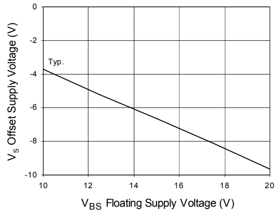
Figure 28. Maximum V_s Negative Offset vs. Supply Voltage
