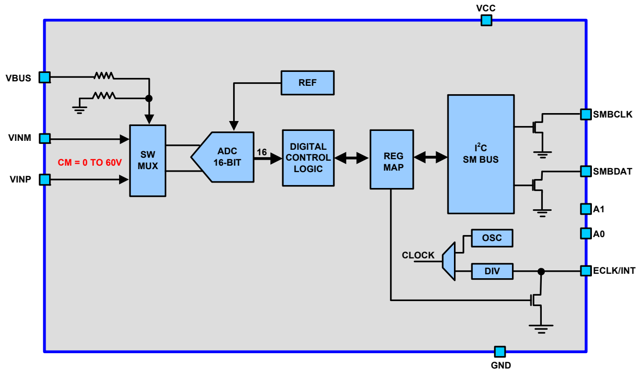
FIGURE 2. BLOCK DIAGRAM
