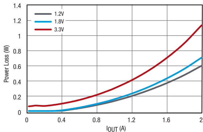
Figure 25. Channel 1 Power Loss at f_{SW} = 440\text{kHz} , V_{IN} = 5\text{V} , No Airflow
