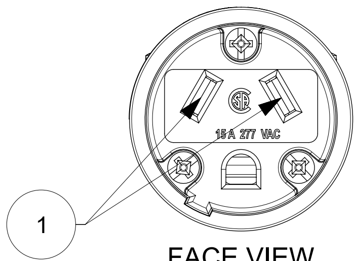
FACE VIEW
