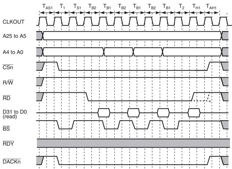
Figure 11.13 Burst ROM Wait Timing
