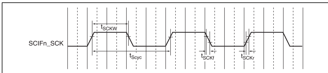
Figure 31.37 SCIFn_SCK Input Clock Timing (n = 0, 1)
