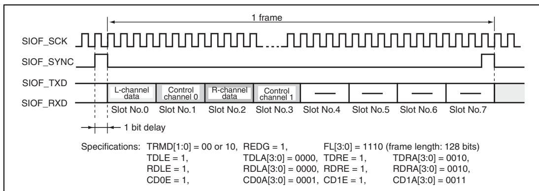
Figure 22.19 Transmit and Receive Timing (16-Bit Stereo Data (4))
