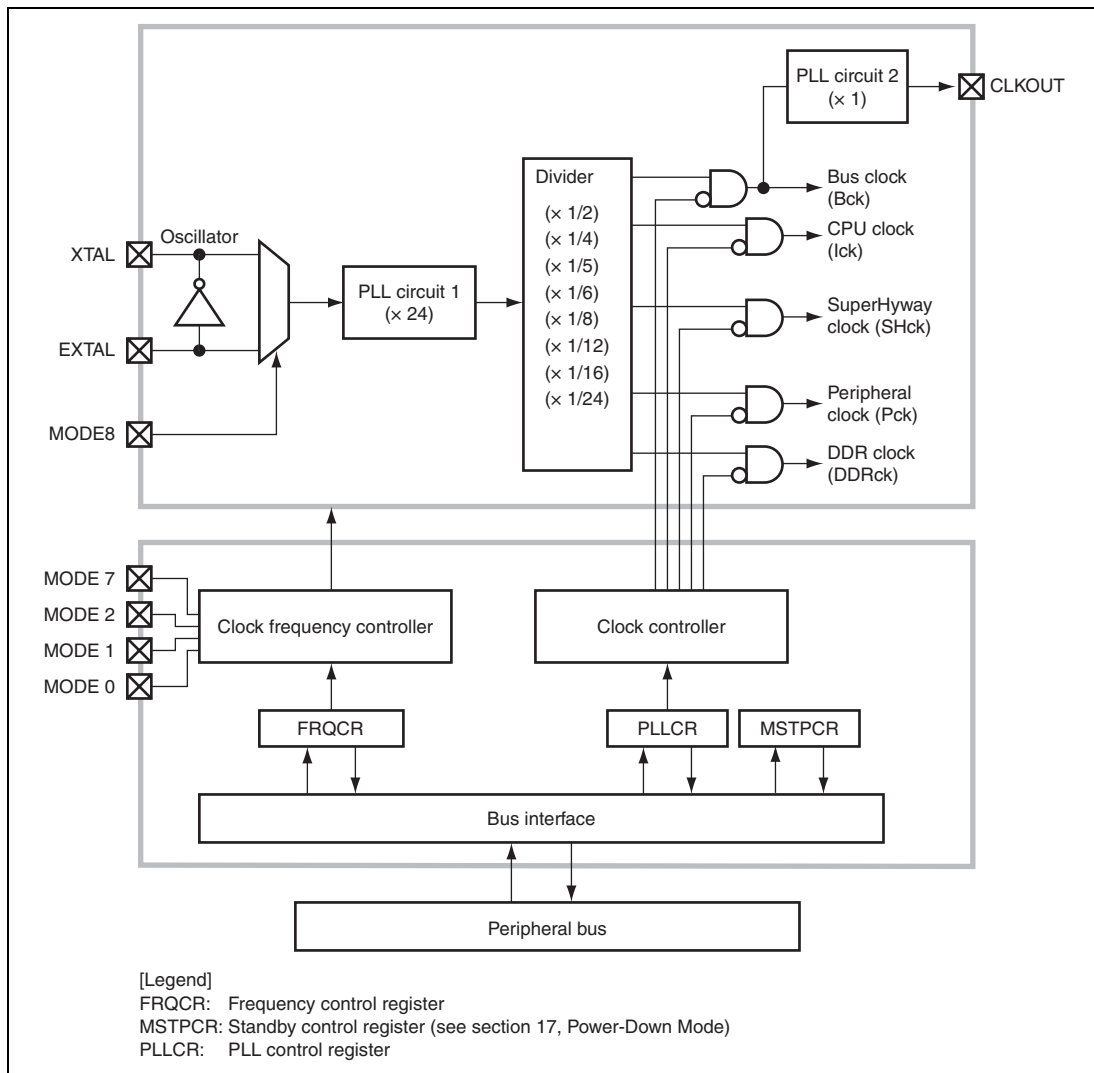
Figure 15.1 Block Diagram of CPG
