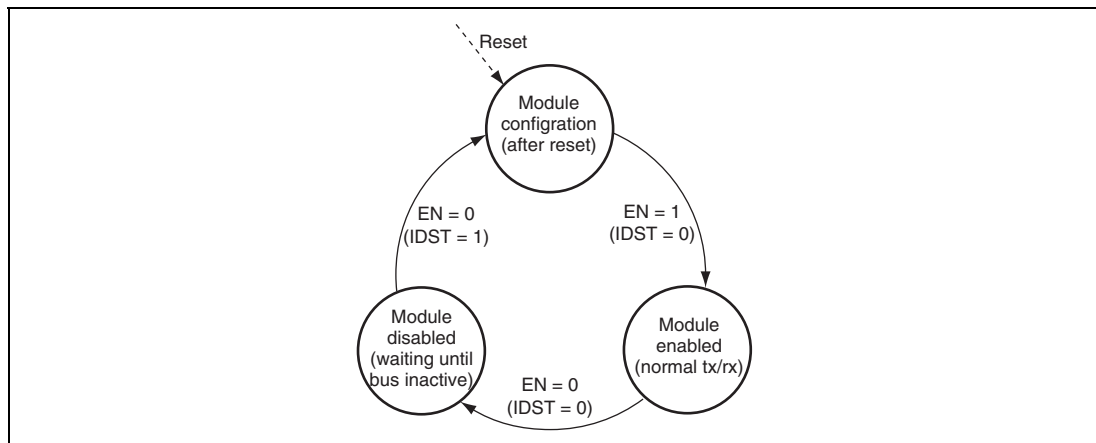
Figure 26.20 Transition Diagram between Operation Modes
