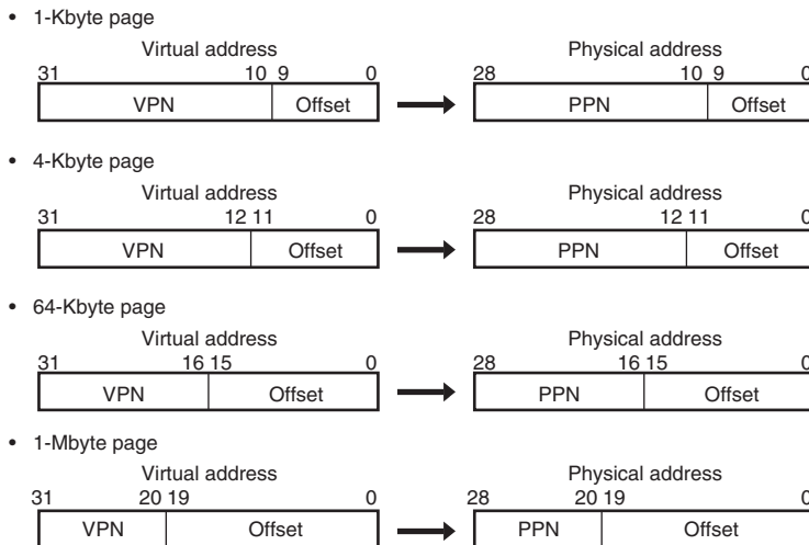
Figure 7.7 Relationship between Page Size and Address Format
