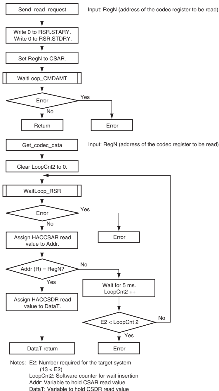
Figure 25.6 Sample Flowchart for Off-Chip Codec Register Read (2)
