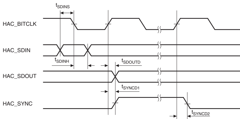
Figure 31.51 HAC Interface Module Signal Timing
