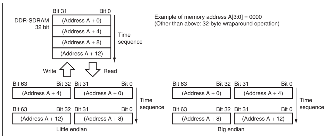
Figure 12.3 Data Alignment in DDR-SDRAM and DDRIF
