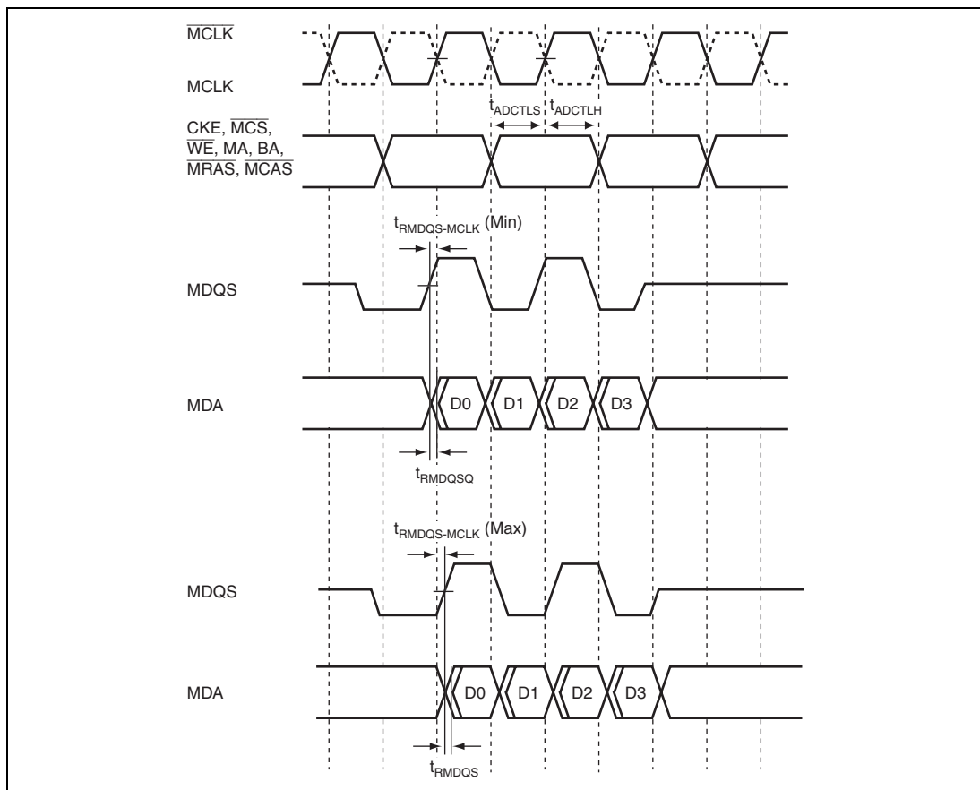
Figure 31.26 Read Timing of DDR-SDRAM (2 Burst Read)
