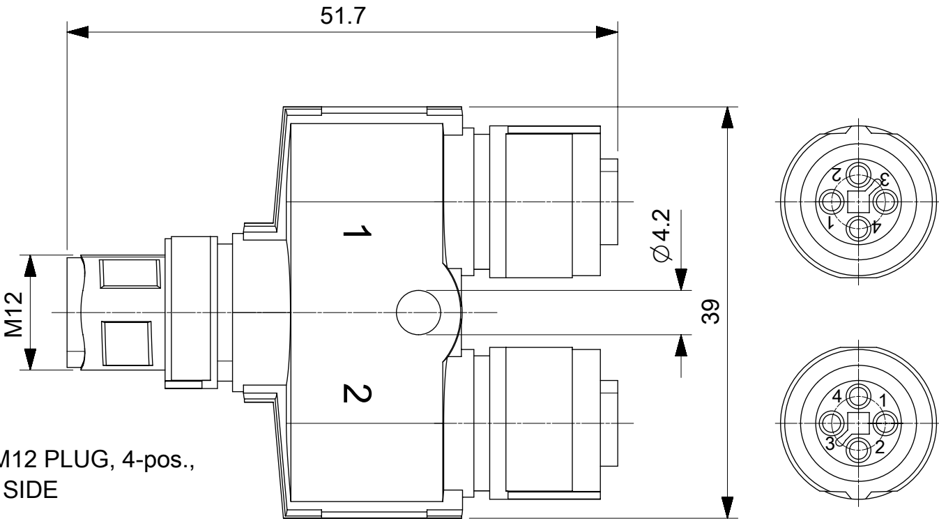
CONNECTOR PIN ASSIGNMENT OF M12 SOCKET, 4-pos.,T-coded, VIEW OF SOCKET SIDE
