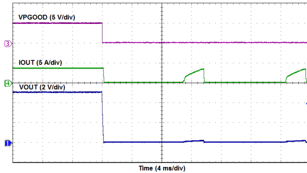
Figure 7-15. Overcurrent Limiting
