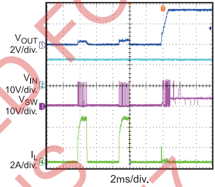
Short Circuit Recovery I_{OUT} = 0A
