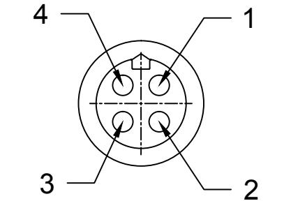
FACE VIEW-MALE INSERT
