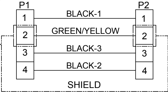
WIRING DIAGRAM
